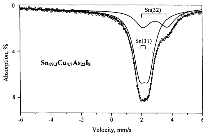
Figure 6. ^{119}\text{Sn} Mössbauer spectrum for \text{Sn}_{19.3}\text{Cu}_{4.7}\text{As}_{22}\text{I}_8 . Solid lines show the fitting doublets. In the top of the spectrum, square brackets show the location of the doublets.
